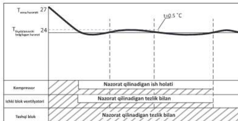
2-rasm. Inverter texnologiyasi turi ( \pm 0,5^{\circ}\text{C} )
