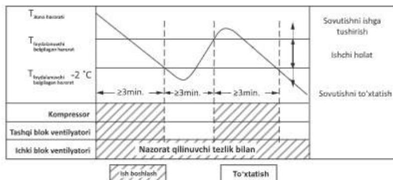
2-rasm. Inverter texnologiyasi turi ( \pm 0,5^{\circ}\text{C} )
